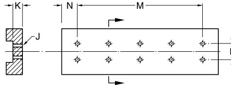
CARRIAGE MOUNTING DIMENSIONS
