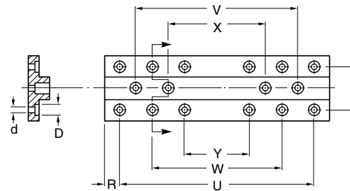
BASE MOUNTING DIMENSIONS
